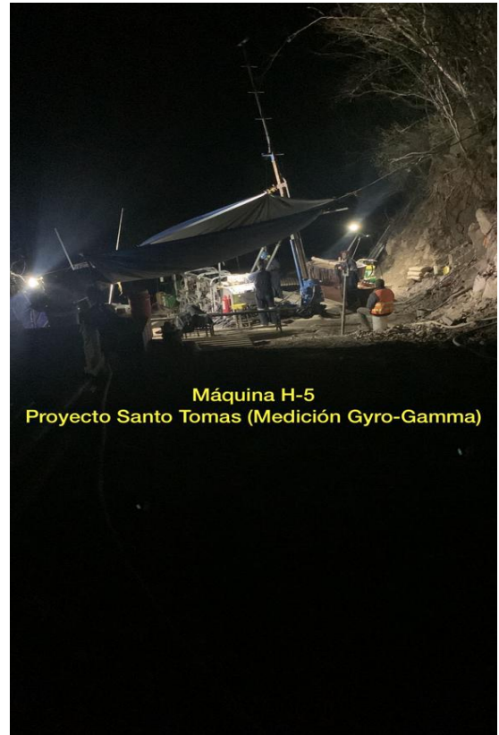
Machine H-5 Santo Tomas Project (Gyro-Gamma Measurement)
